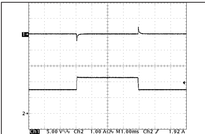
Figure 5: Output voltage response to step-change in load current (66% - 100% - 66% of I out (max); dl/dt = 0.1 A/μs). Load cap: 15 μF tantalum cap and 1 μF ceramic cap. Ch 1: V out (5 V/div), Ch 2: I out (1 A/div).
