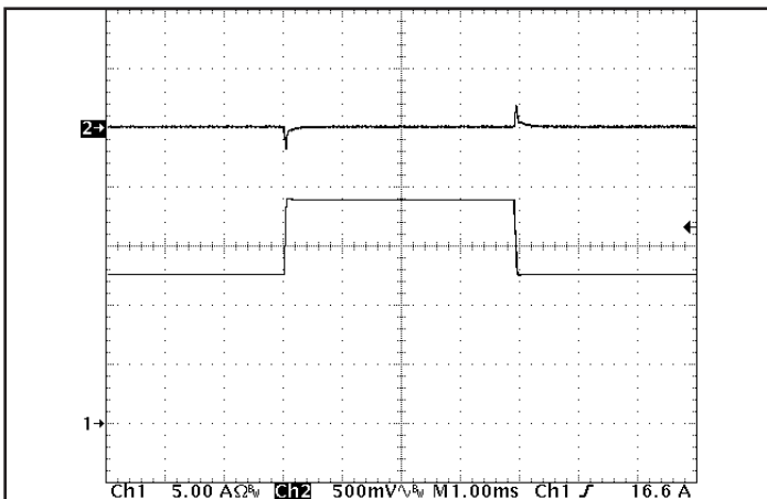
Figure 5: Output voltage response to step-change in load current (66% -100% -66% of I out (max); dI/dt = 0.1 A/μs). Load cap: 15 μF tantalum cap and 1 μF ceramic cap. Ch 1: I out (5 A/div), Ch 2: V out (500 mV/div).
