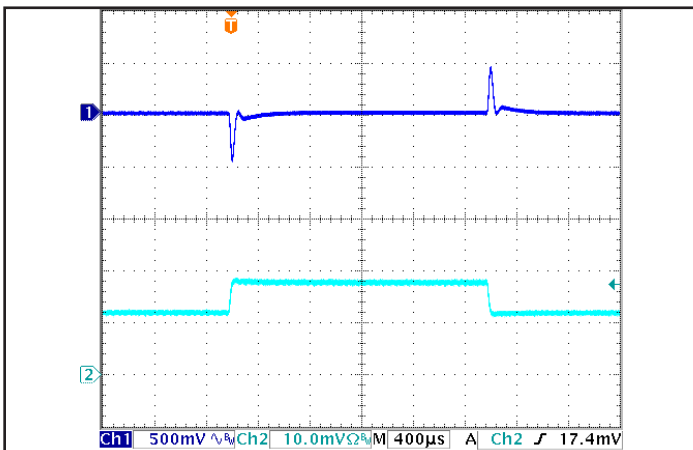
Figure 5: Output voltage response to step-change in load current (66% - 100% - 66% of I out (max); dl/dt = 0.1 A/μs). Load cap: 15 μF tantalum cap and 1 μF ceramic cap. Ch 1: V out (500 mV/div), Ch 2: I out (5 A/div).
