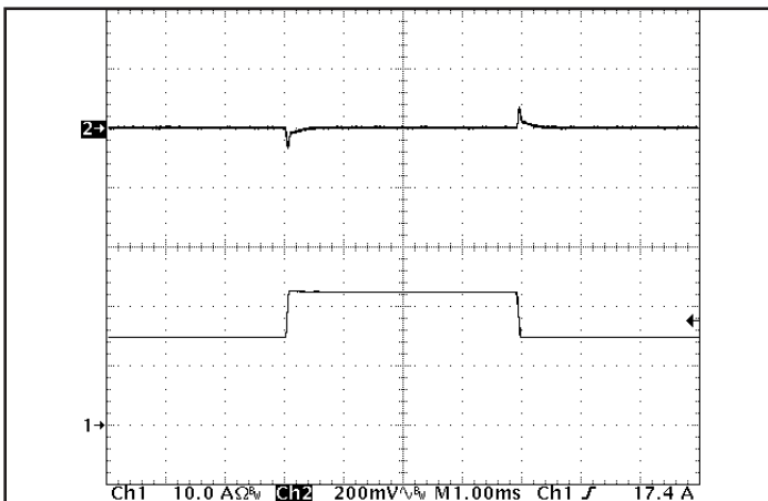
Figure 5: Output voltage response to step-change in load current (66% -100% -66% of I out (max); dI/dt = 0.1 A/μs). Load cap: 15 μF tantalum cap and 1 μF ceramic cap. Ch 1: I out (10 A/div), Ch 2: V out (200 mV/div).
