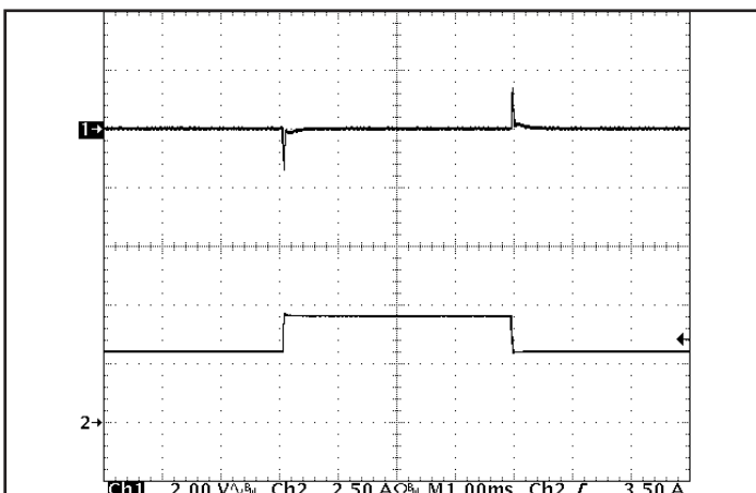
Figure 5: Output voltage response to step-change in load current (66% - 100% - 66% of I out (max); dl/dt = 0.1 A/μs). Load cap: 15 μF tantalum cap and 1 μF ceramic cap. Ch 1: V out (2 V/div), Ch 2: I out (2.5 A/div).
